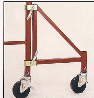
Part No. 0172-0105 - 18"W Outrigger
